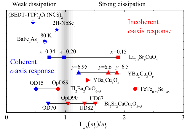
FIG. 3 (color online). ab -plane scattering rate \Gamma_{ab}(\omega_0) divided by \omega_0 . \omega_0 is the frequency that accounts for 30% of the intraband SW. The gray bar denotes the region close to \Gamma_{ab}(\omega_0) \sim \omega_0 . The left and right sides of this region represent the weak and strong dissipation regimes, respectively. The majority of the materials with strong ab -plane dissipation exhibit incoherent c -axis response (red symbols). The latter is defined by the suppression of the low-energy SW in \sigma_c(\omega) at low T concomitant with d\rho_c/dT < 0 . The majority of the materials with weak ab -plane dissipation reveal coherent c -axis behavior (blue symbols): the enhancement of the low-energy SW in \sigma_c(\omega) and d\rho_c/dT > 0 . Data points: \text{FeTe}_{0.55}\text{Se}_{0.45} (Ref. [16]), \text{BaFe}_2\text{As}_2 (Refs. [38,39]), 2H\text{-NbSe}_2 (Ref. [27]), (\text{BEDT-TTF})_2\text{Cu}(\text{NCS})_2 (Refs. [29,37]), cuprates (Refs. [33–36,41–44]). (UD, underdoped; OpD, optimally doped; OD, overdoped. The number denotes T_c of each compound.)
